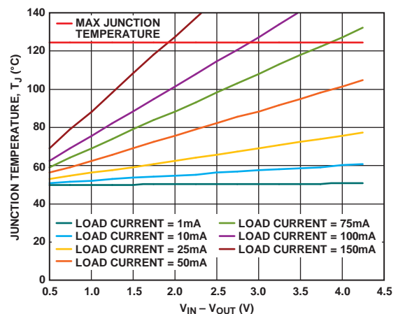
Figure 35. 0 mm 2 of PCB Copper, T_A = 50^\circ\text{C}
