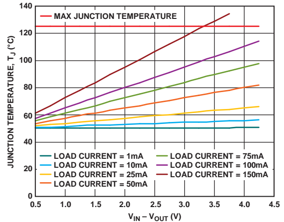
Figure 33. 500 mm 2 of PCB Copper, T_A = 50^\circ\text{C}
