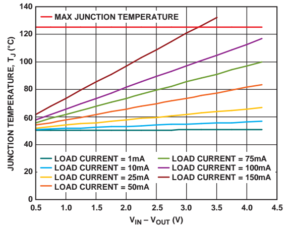
Figure 34. 100 mm 2 of PCB Copper, T_A = 50^\circ\text{C}
