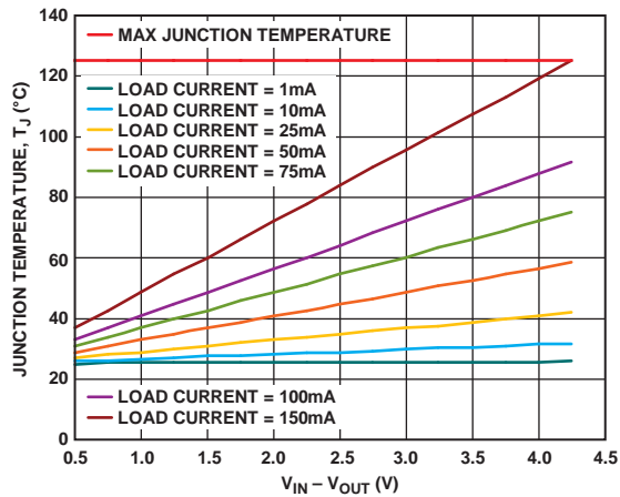
Figure 31. 100 mm 2 of PCB Copper, T_A = 25^\circ\text{C}
